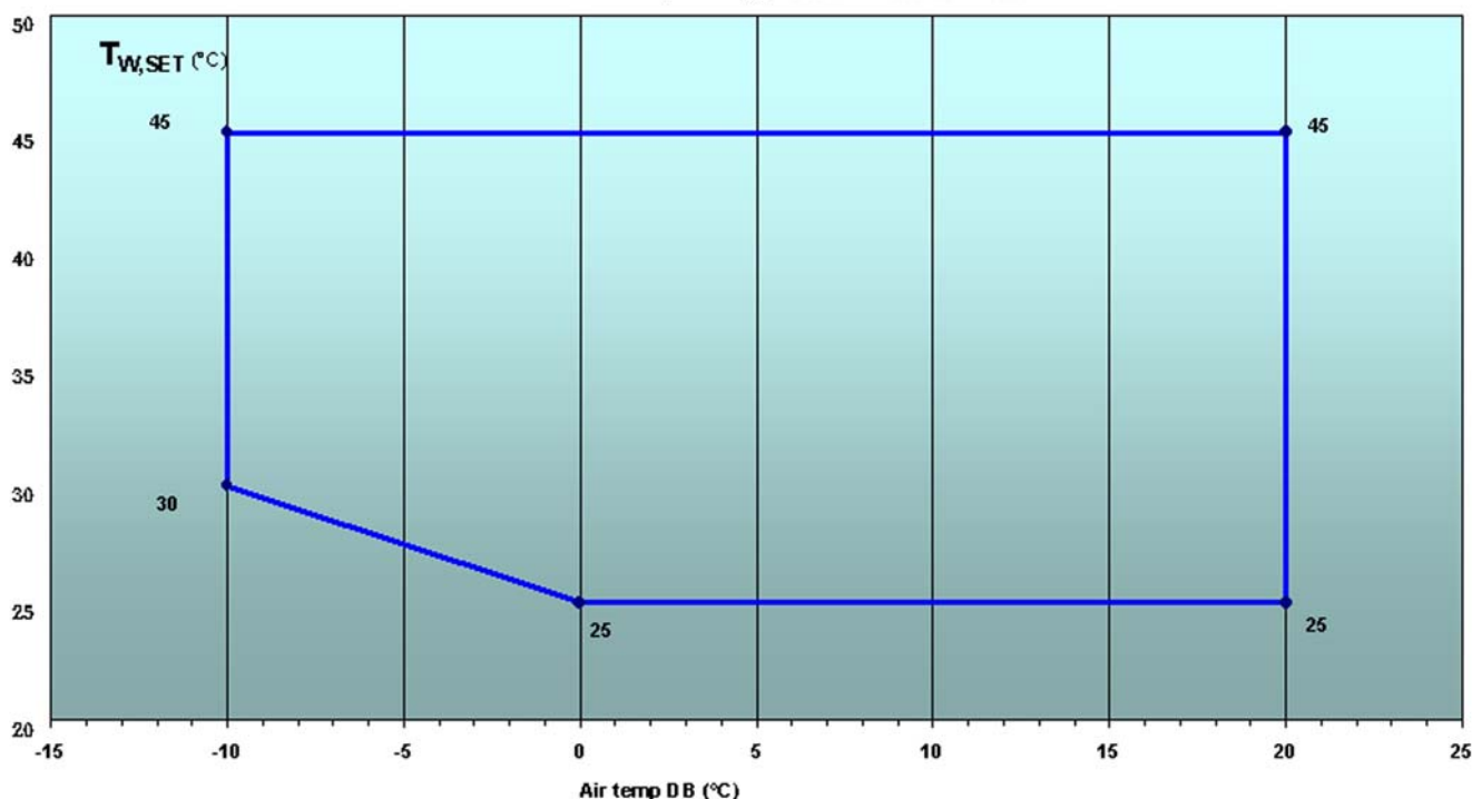
Operation Limits T_{W,SET} @ 1380 l/h water flow rate
